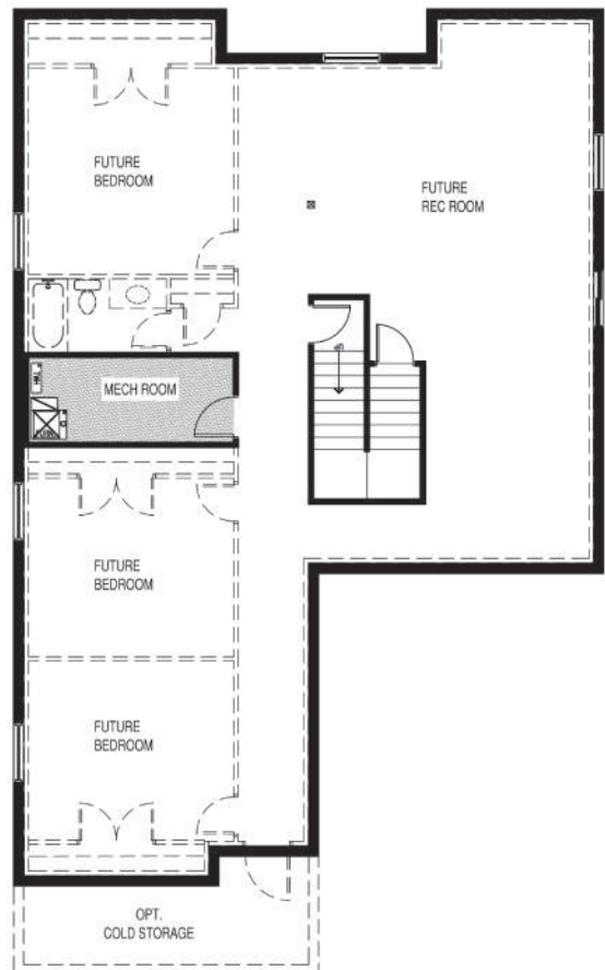
BASEMENT FLOOR | 1,790 SQ. FT.
