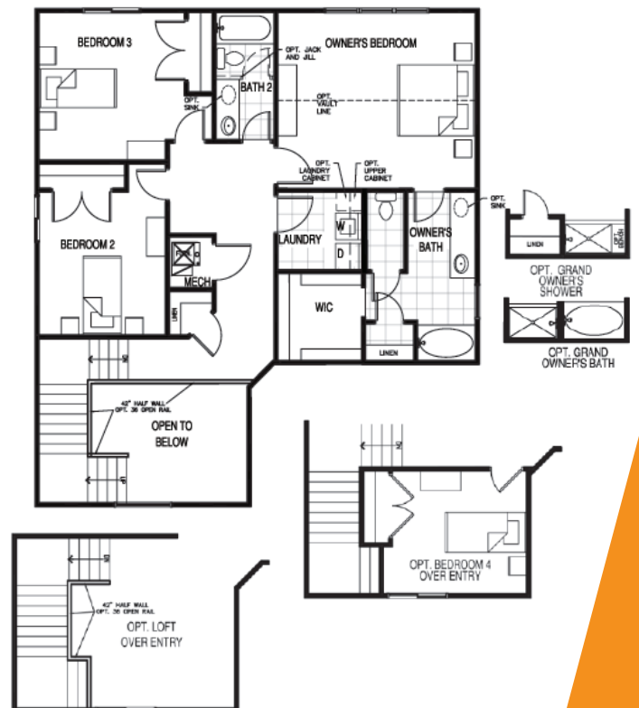
UPPER FLOOR | 1,363 SQ. FT.
